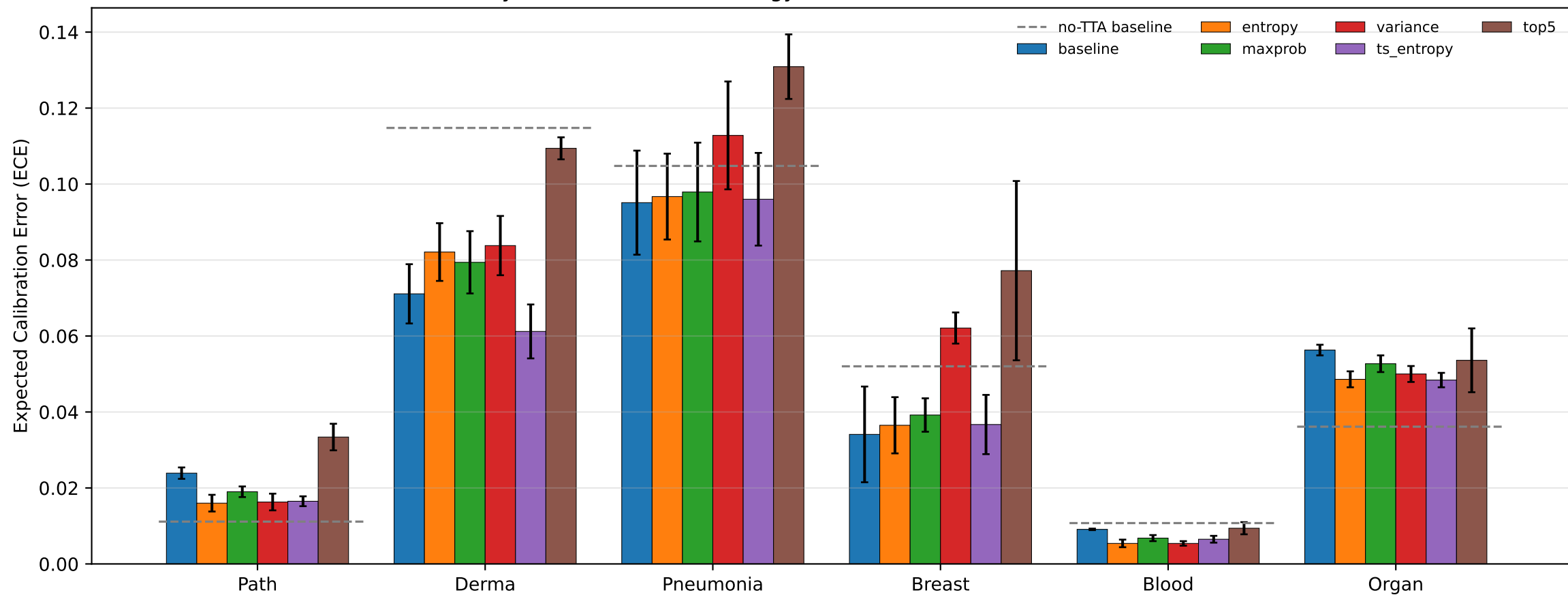
ECE by dataset and TTA strategy — ResNet-18 (mean \pm std over seeds)
