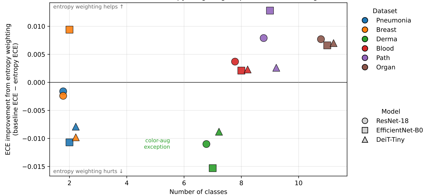
Calibration mechanism: entropy weighting helps more as classes grow
