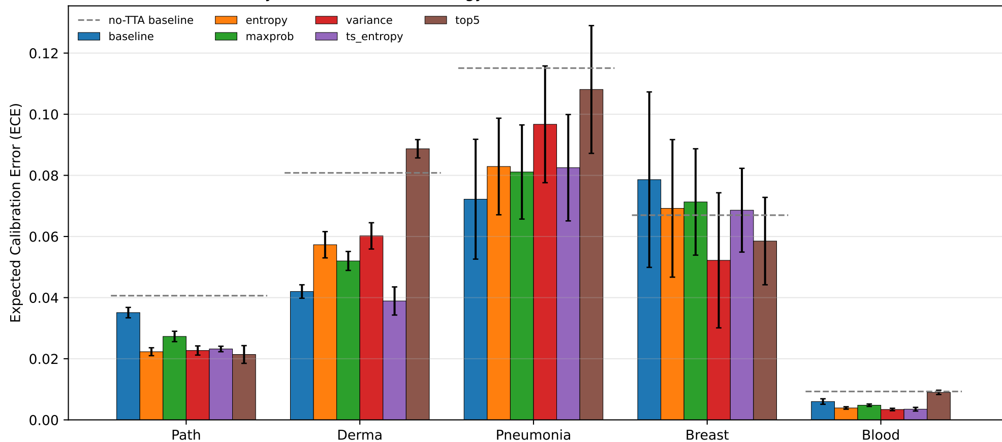
ECE by dataset and TTA strategy — EfficientNet-B0 (mean \pm std over 3 seeds)
