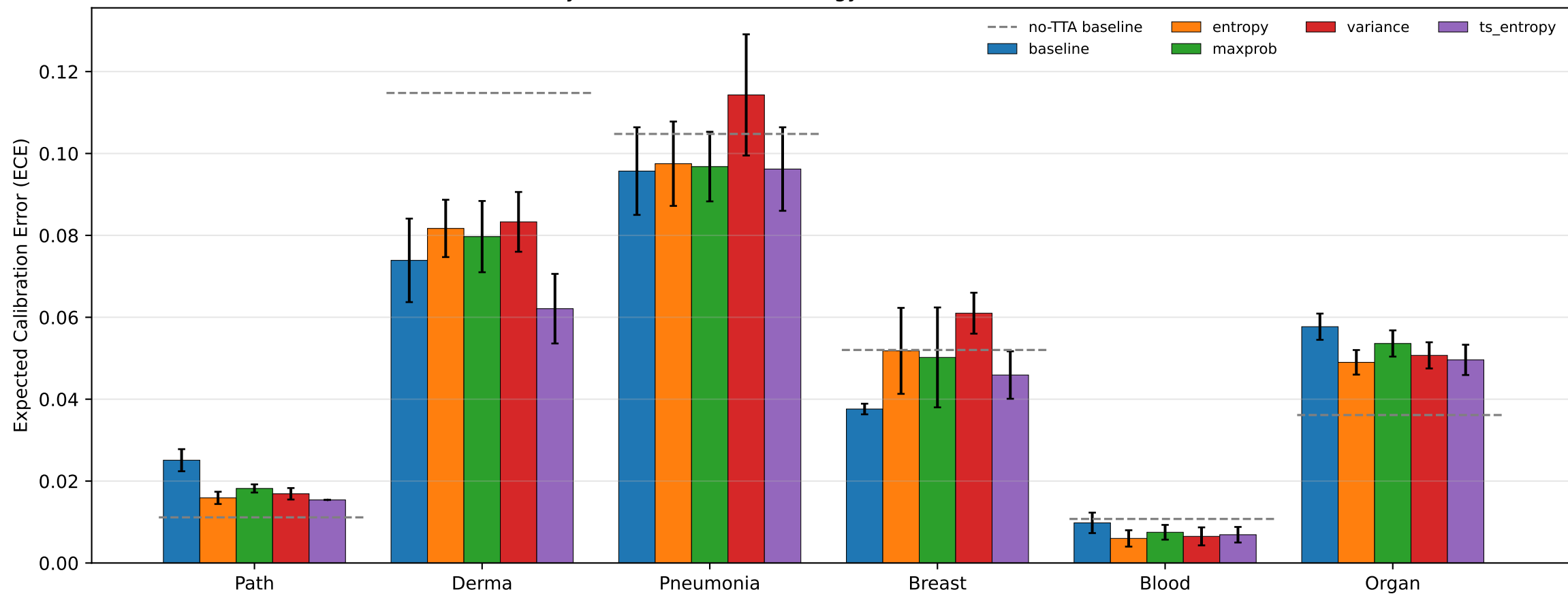
ECE by dataset and TTA strategy (mean \pm std over 3 seeds)
