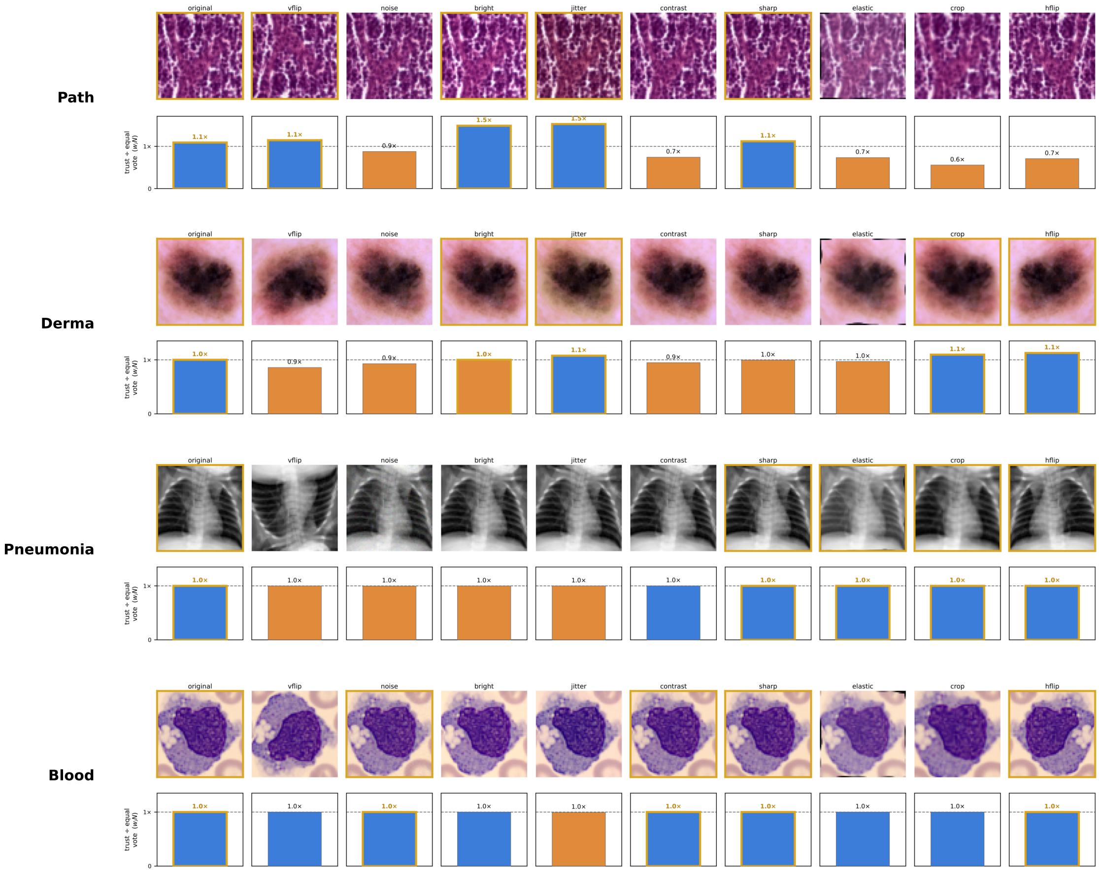
Figure 1 (ResNet-18), sample 3
