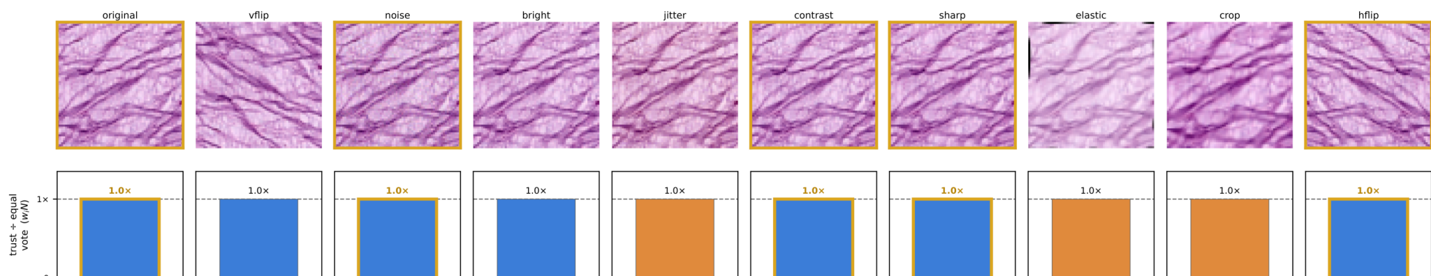
Path sample 6
