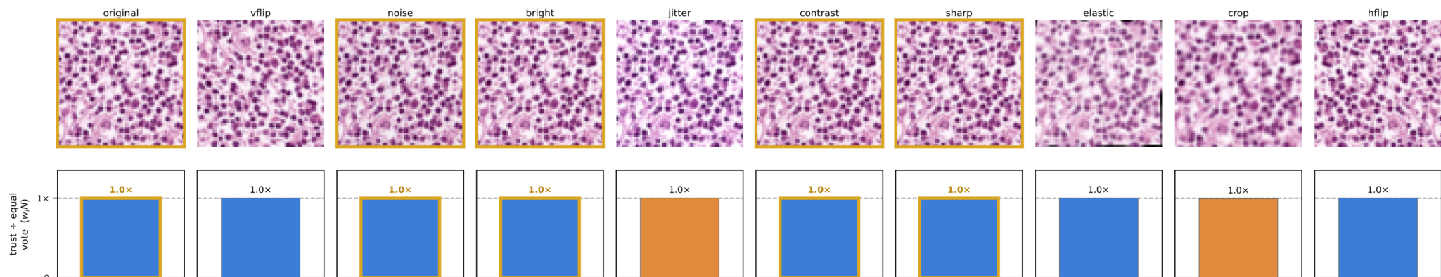
Path sample 4
