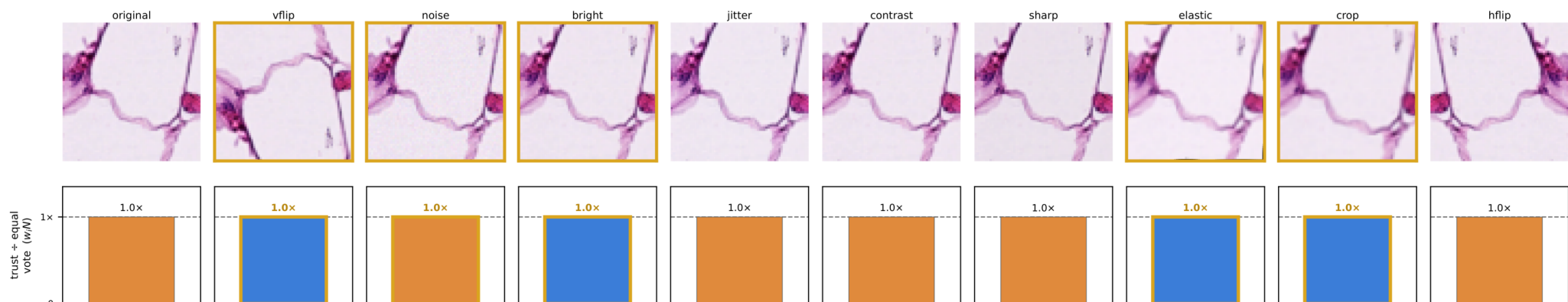
Path sample 5
