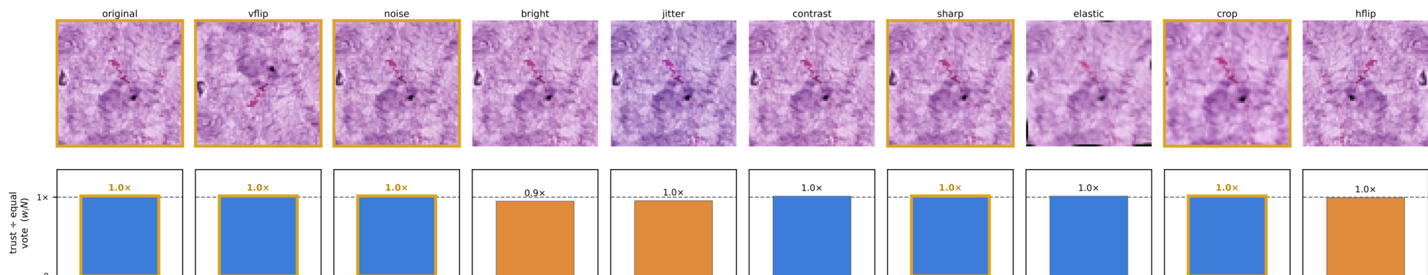
Path sample 2
