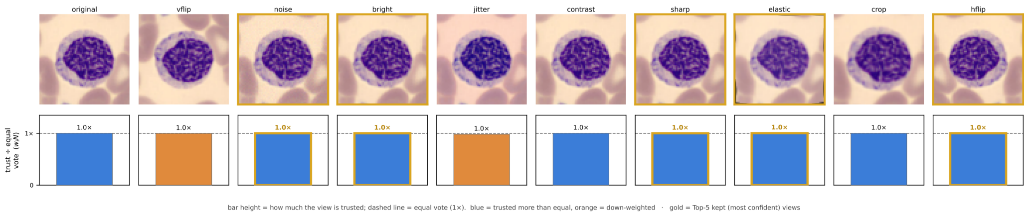
Augmentation Confidence Strip — BloodMNIST (Blood Cell Microscopy) - Sample 6 (idx=163)
