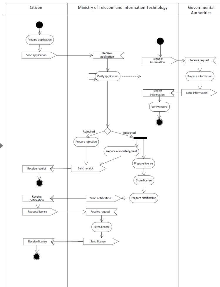
Re-engineered process “To-be model”
