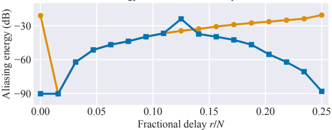
Energy outside \pm H of the impulse
