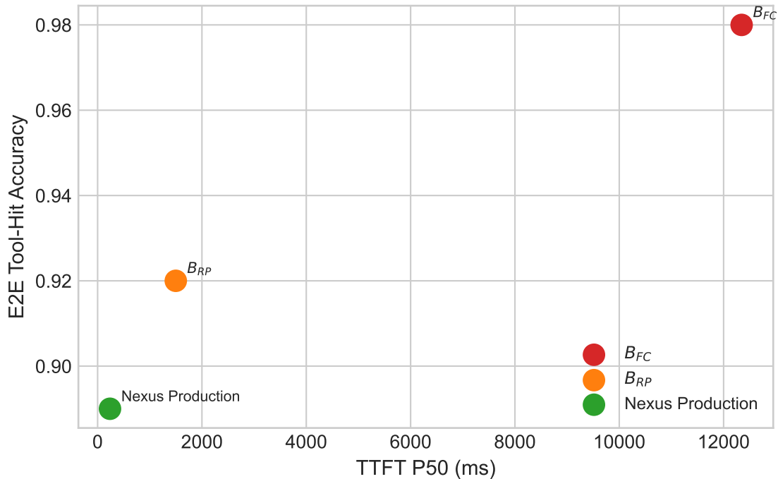
Accuracy--Latency Pareto Frontier
