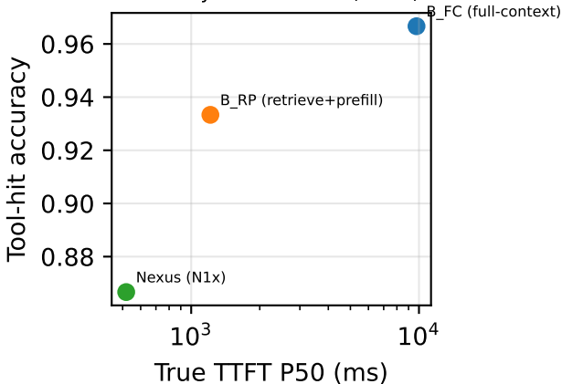
Accuracy vs. true TTFT (n=30)
