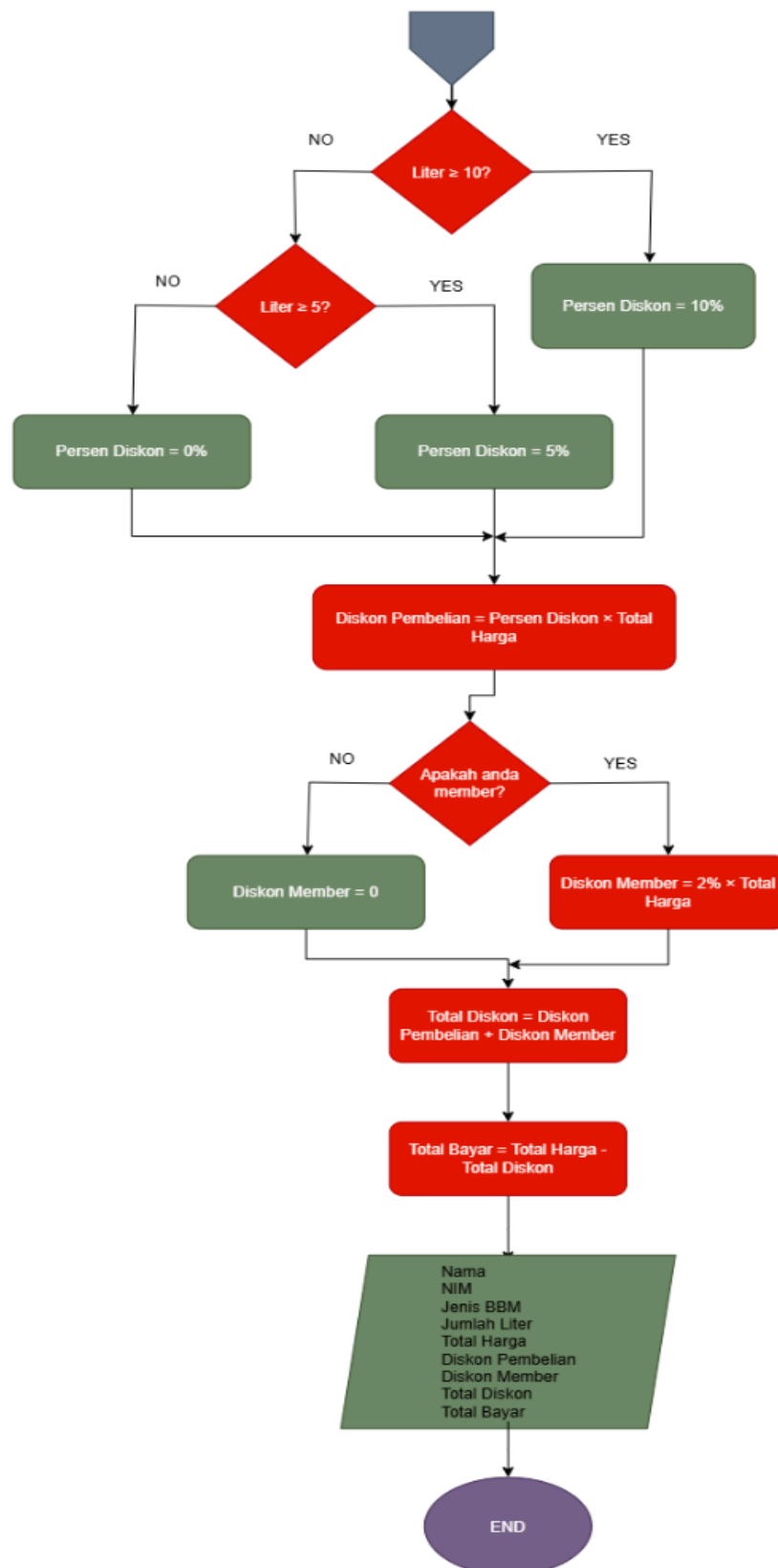
Gambar 1.3 Flowchart
