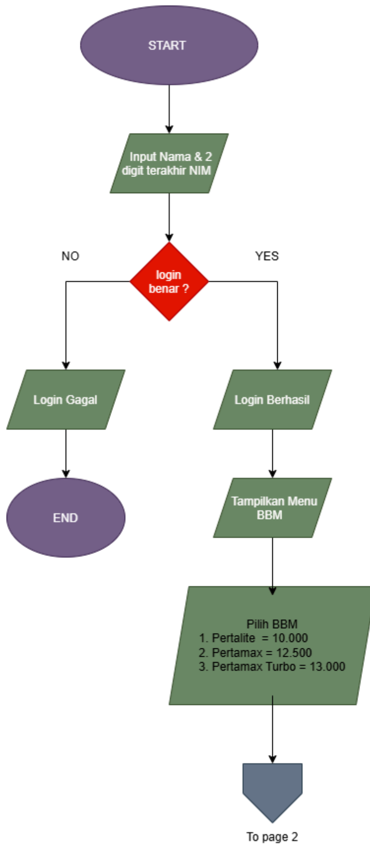
Gambar 1.1 flowchart
