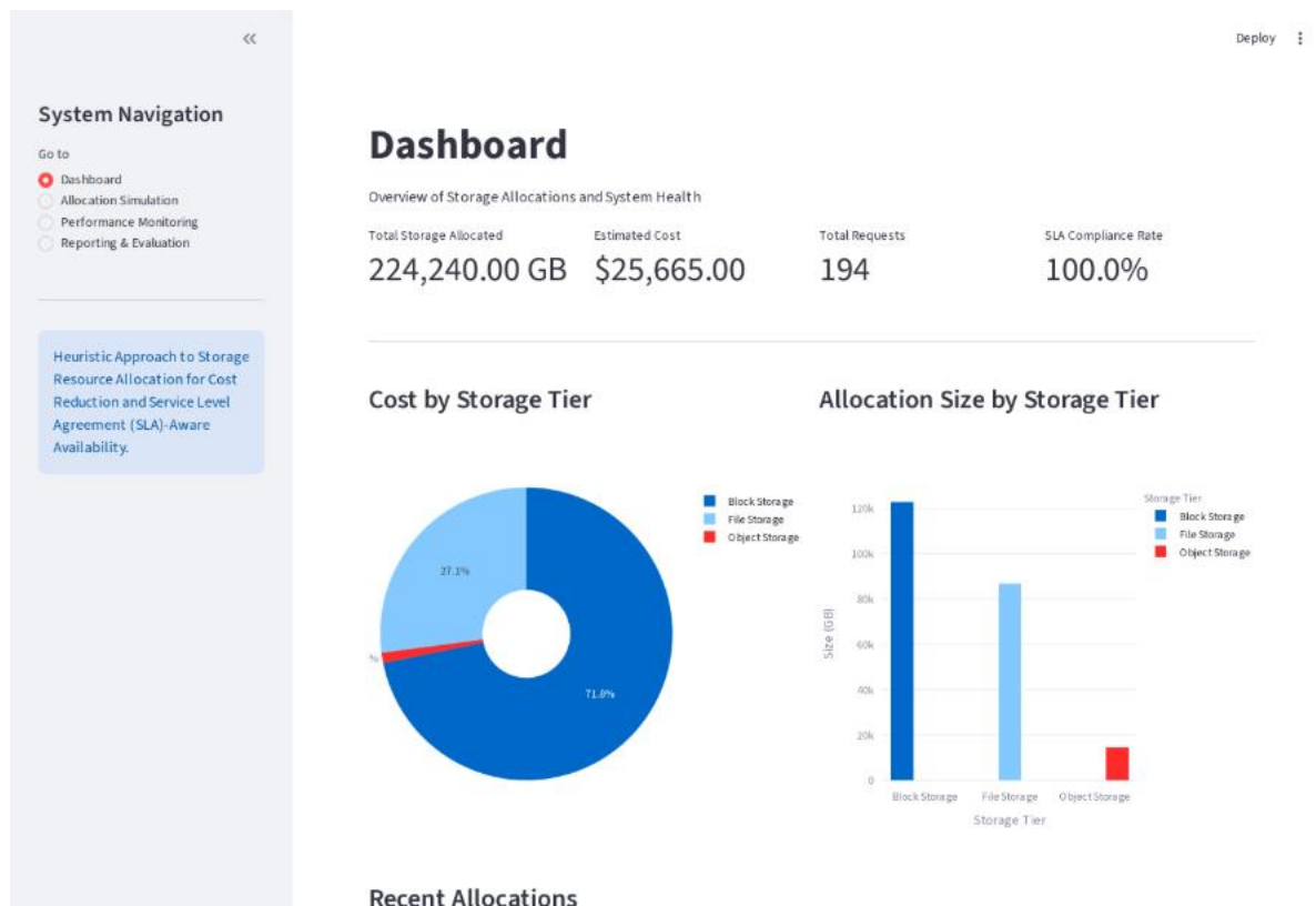
Figure 4.1: Streamlit Executive Dashboard View displaying system KPI metric cards and Plotly distribution charts
