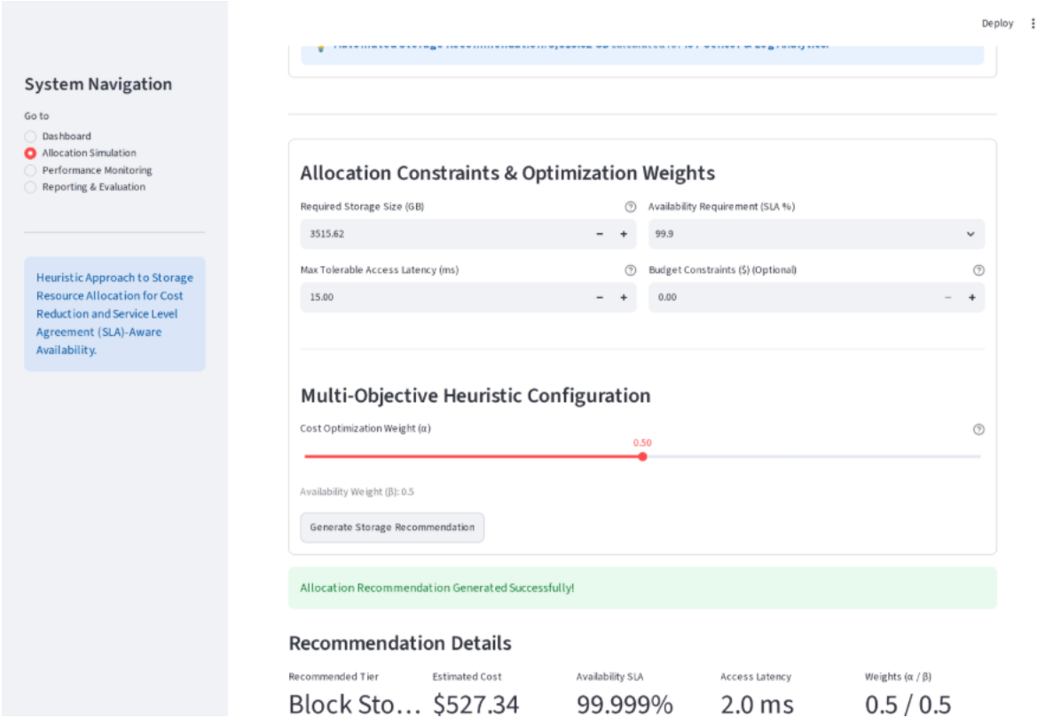
Figure 4.2: Storage Resource Allocation Simulation View displaying the Automatic Storage Size Suggestion Engine and baseline comparative analysis
