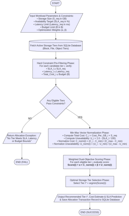
Figure 3.6: Flowchart logic of the core multi-objective storage allocation algorithm
