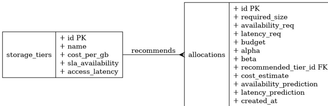
Figure 3.4: Entity Relationship Diagram showing one-to-many relationship between storage_tiers and allocations tables.
