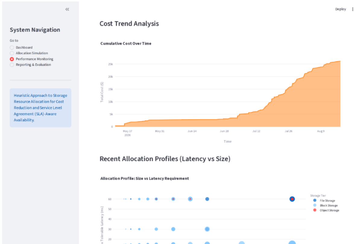
Figure 4.3: Tier Performance Monitoring View showing cumulative storage growth, cost trends, and profile distribution
