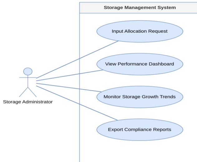
Figure 3.3: Use case diagram showing Storage Administrator interactions with the system.
