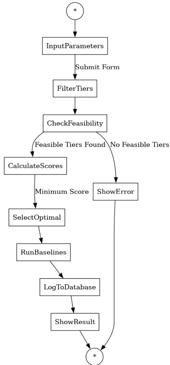
Figure 3.5: Activity diagram showing the operational logic flow for generating storage recommendations.
