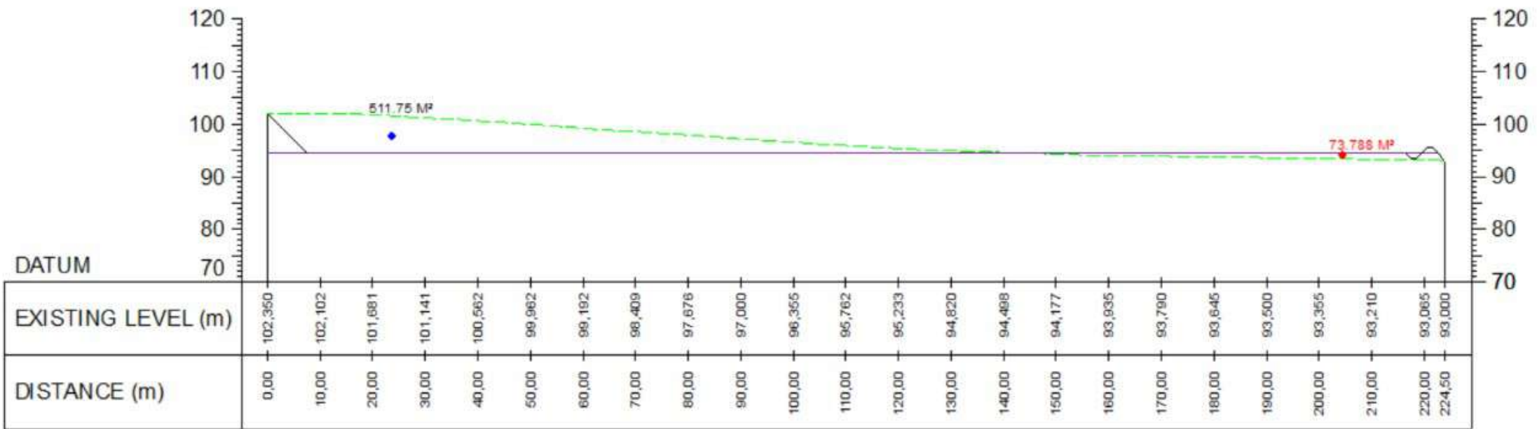
SECTION E
