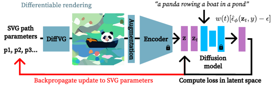
Figure 3.2: SDS optimization loop in VectorFusion [21].
