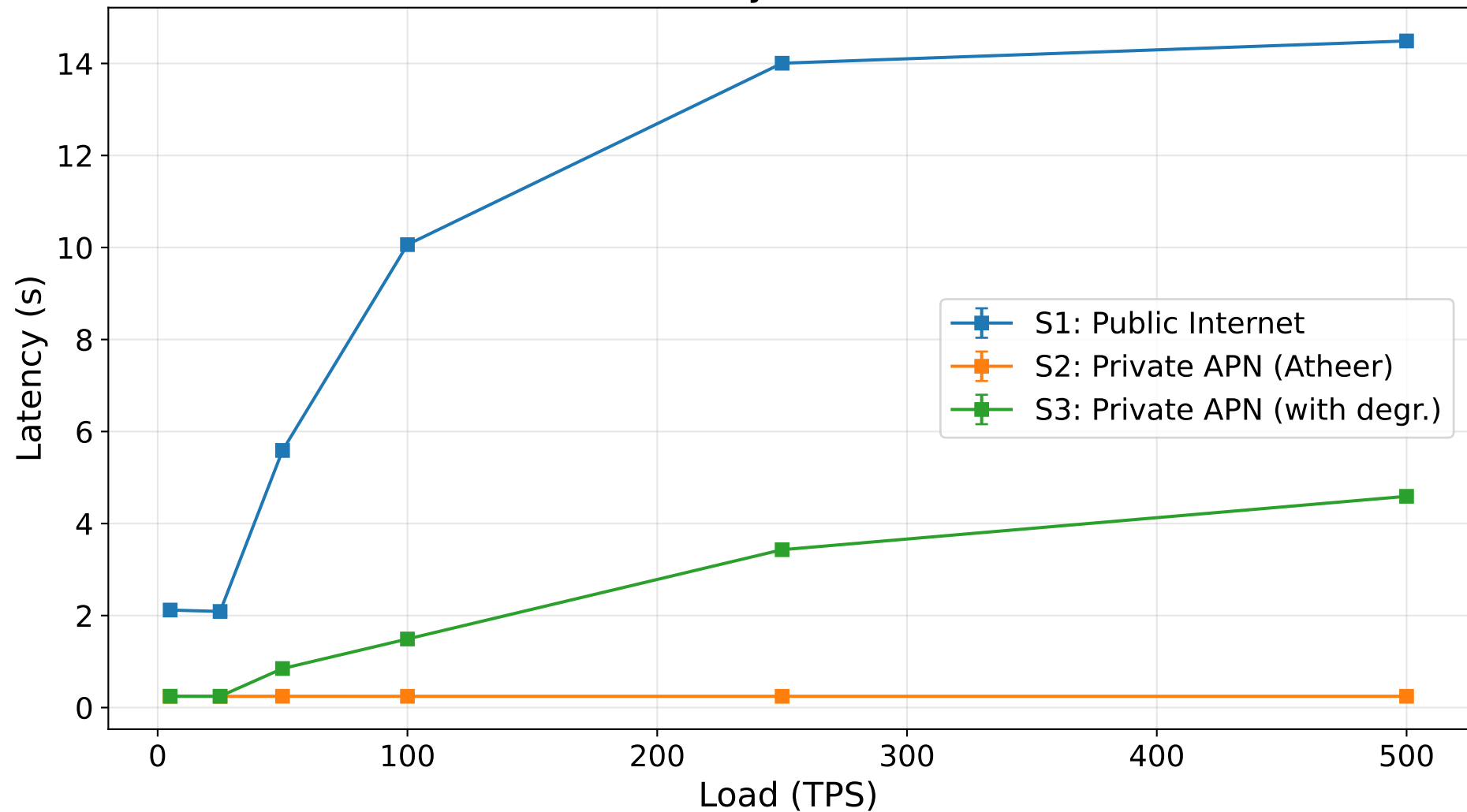
P95 End-to-End Latency vs Load (Mean \pm 95% CI)
