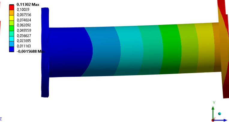
B: FMmin Adapter_Amplitude_Deformation 2 Expression: D3min-D1min Unit: mm Deformation Scale Factor: 200,
