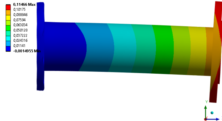
B: FMmin Adapter_Amplitude_Deformation Expression: D2min-D1min Unit: mm Deformation Scale Factor: 200,
