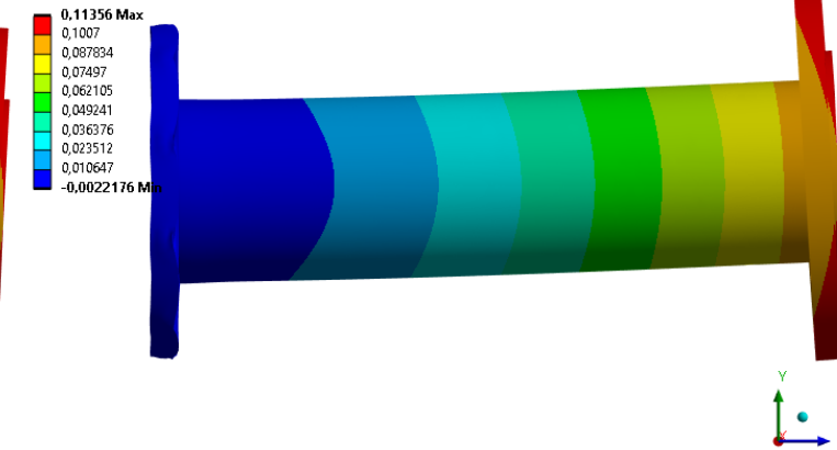
A: FMmax Adapter_Amplitude_Deformation 3 Expression: D3-D1 Unit: mm Deformation Scale Factor: 200,
