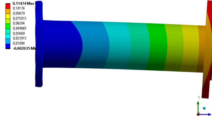
A: FMmax Adapter_Amplitude_Deformation 2 Expression: D2-D1 Unit: mm Deformation Scale Factor: 200,
