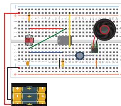
Breadboard Prototype
