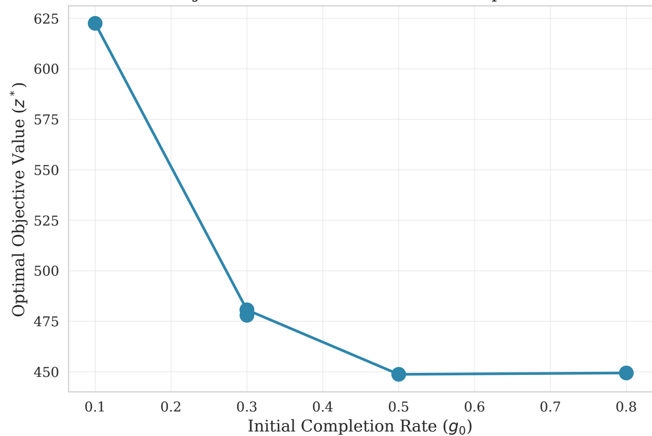
Objective Value vs. Initial State Completion
