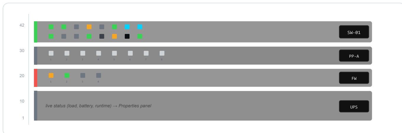
Fig. 3 — Rack front on white viewport. The vertical stripe on the left is the SNMP status (green ok · amber not polled yet · red error · grey not configured). Port LEDs are small squares (green active · amber idle · red error · grey down or never measured · dark grey no link across three Verifies · near-black shut by hand · blue LAG ) with the port number below. Device data (IP, status, UPS runtime...) is read in the Properties panel .
