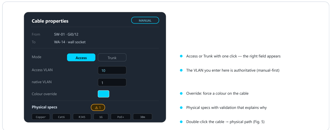
Fig. 4 — The cable editor: endpoints (read-only), Access/Trunk mode, VLANs, colour override, physical specs with the ⚠ warning badge.
