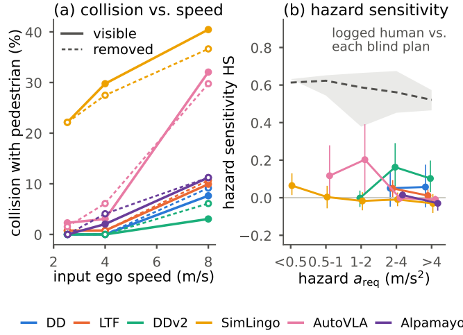
Fig. 3. Collision and hazard sensitivity. (a) Contact with the pedestrian’s logged future at the logged and counterfactual input speeds; solid: visible, dashed: removed. (b) HS against a_{\text{req}} (mean, 95% CI, bins with \geq 8 units). Dashed: the logged human trajectory scored against each policy’s blind plan, averaged; band: range over policies.
