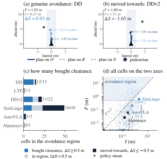
Fig. 2. The two axes. (a) Genuine avoidance: with the pedestrian in view ( X^O , solid) DiffusionDrive stays short of its logged future (dashed from the star), while blind to it ( X^R , dashed) it reaches it. X^N gives I . (b) Moved towards: DiffusionDriveV2 plans further with the pedestrian than without. (c) Cells in the avoidance region ( F \geq 0.5 m, F > I ) per policy, by \Delta S : blue \geq 0.5 m, navy \leq -0.5 m, grey between. Label: blue over all. (d) All 1,476 cells (246 scenes \times six policies) on the axes of (3), by policy, with means.
