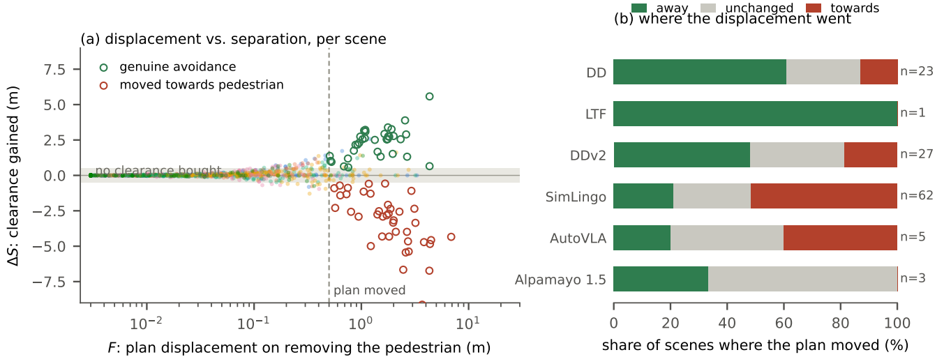
Fig. 4. Displacement is not avoidance. (a) Every policy–scene cell of the 246 NAVSIM Singapore scenes: the plan displacement caused by removing the pedestrian ( F , log scale) against the clearance it buys against the pedestrian’s logged future ( \Delta S ). Below the F = 0.5 m threshold the cloud is pinned to \Delta S = 0 ; above it the points fan out almost symmetrically. Circled: cells meeting all three conditions for genuine avoidance (green) and cells whose plan moved towards the pedestrian (red). (b) Among the cells where the plan moved, where the displacement went.
