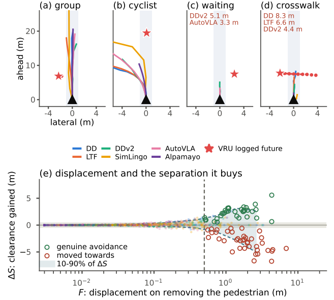
Fig. 5. Four right-hand-drive cases, and displacement against the separation it buys. (a–d) Ego at the origin, its corridor shaded, the VRU’s logged future dashed from the star; every policy receives the frame’s logged navigation, so the turns are commanded. (a) Clearances 0.3–0.9 m. (b) SimLingo passes at 3.2 m, the other five at 6.7–10 m. (c, d) The departing policies and their planned distances are named in the panel; Boston departure rates are DiffusionDriveV2 81%, AutoVLA 9%, DiffusionDrive 2.8%. (e) Every policy–scene cell of the 246 Singapore scenes: F against \Delta S ; band: the 10–90% spread of \Delta S per F bin; dashed line: F = 0.5 m.
