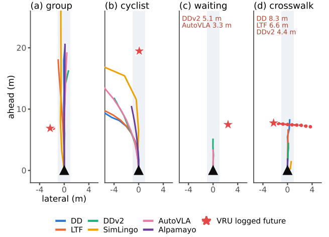
Fig. 4. Four right-hand-drive cases. Ego at the origin, its corridor shaded, the VRU’s logged future dashed from the star. (a) Group at the lane edge, clearances 0.3–0.9 m. (b) Cyclist at a left turn; SimLingo passes at 3.2 m, the other five at 6.7–10 m. (c, d) Human waiting; the departing policies and their planned distances are named in the panel. Boston departure rates: DiffusionDriveV2 81%, AutoVLA 9%, DiffusionDrive 2.8%.
