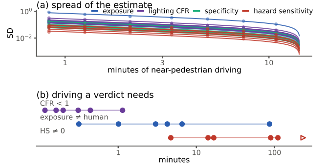
Fig. 4. How much driving a verdict costs. One frame is 5s of near-pedestrian driving. (a) Spread of each exam’s estimate against sample size, with its fitted law; one line per policy. (b) Driving needed to settle each verdict, one dot per policy; values beyond the axis are off scale.
