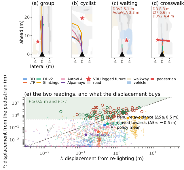
Fig. 2. Four right-hand-drive cases, and displacement against the separation it buys. (a–d) Ego at the origin, the vulnerable road user’s (VRU) logged future dashed from the star, and DiffusionDriveV2’s own BEV semantic head as the background; every policy receives the frame’s logged navigation, so the turns are commanded. (a) Clearances 0.3–0.9 m. (b) SimLingo passes at 3.2 m, the other five at 6.7–10 m. (c, d) The departing policies and their planned distances are named in the panel. (e) Every policy–scene cell of the 246 Singapore scenes on the two axes of (3), with the policy means; rings mark cells whose displacement bought ( \Delta S \geq 0.5 m) or cost ( \Delta S \leq -0.5 m) clearance; shaded: the avoidance region F \geq 0.5 m, F > I .
