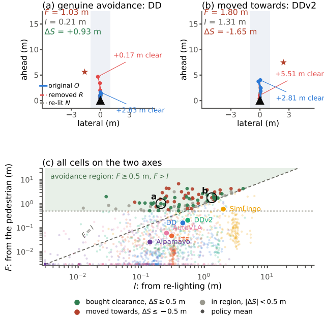
Fig. 2. The two axes, on two cells and on all of them. (a) A cell counted as genuine avoidance: DiffusionDrive’s plan with the pedestrian in view ( X^O , solid) stays short of the pedestrian’s logged future (dashed from the star), while the pedestrian-blind plan ( X^R , dashed) reaches it; the re-lit plan ( X^N ) gives I . (b) A cell in which the plan moved towards the pedestrian: DiffusionDriveV2 plans further with the pedestrian in view than without it. (c) Every policy–scene cell of the 246 Singapore scenes on the two axes of (3), with the policy means and the cells of (a) and (b). Inside the avoidance region ( F \geq 0.5 m, F > I , shaded) cells are coloured by what the displacement bought: green \Delta S \geq 0.5 m, red \Delta S \leq -0.5 m, grey in between; outside it, by policy.
