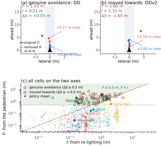
Fig. 2. The two axes, on two cells and on all of them. (a) A cell counted as genuine avoidance: DiffusionDrive’s plan with the pedestrian in view ( X^O , solid) stays short of the pedestrian’s logged future (dashed from the star), while the pedestrian-blind plan ( X^R , dashed) reaches it; the re-lit plan ( X^N ) gives I . (b) A cell in which the plan moved towards the pedestrian: DiffusionDriveV2 plans further with the pedestrian in view than without it. (c) Every policy-scene cell of the 246 Singapore scenes on the two axes of (3), with the policy means and the cells of (a) and (b); rings mark cells whose displacement bought ( \Delta S \geq 0.5 m) or cost ( \Delta S \leq -0.5 m) clearance; shaded: F \geq 0.5 m, F > I .
