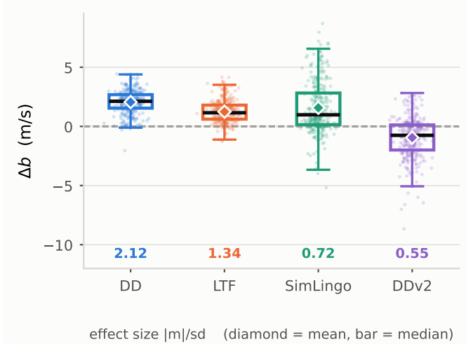
Fig. 1. Why we do not report a mean alone. Distribution of \Delta b under the full-image night rendering, one point per event ( n=312 ). DiffusionDrive and LTF show a concentrated shift—narrow box, mean on top of median. SimLingo’s interquartile range is three times wider, its mean (diamond) sits well above its median (bar), and the points separate into a group near zero and a group above +3; DiffusionDriveV2’s box straddles zero. The effect size |\mu|/\sigma below each box is the number to read.
