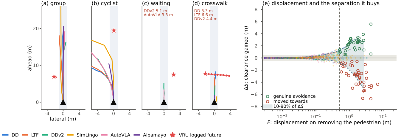
Fig. 4. Four right-hand-drive cases, and displacement against the separation it buys. (a–d) Ego at the origin, its corridor shaded, the VRU’s logged future dashed from the star; every policy receives the frame’s logged navigation, so the turns are commanded. (a) Clearances 0.3–0.9 m. (b) SimLingo passes at 3.2 m, the other five at 6.7–10 m. (c, d) The departing policies and their planned distances are named in the panel; Boston departure rates are DiffusionDriveV2 81%, AutoVLA 9%, DiffusionDrive 2.8%. (e) Every policy–scene cell of the 246 Singapore scenes: F against \Delta S ; band: the 10–90% spread of \Delta S per F bin; dashed line: F = 0.5 m.
