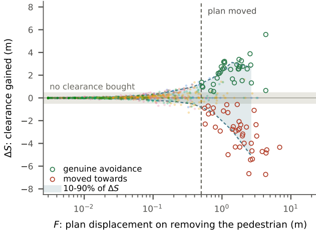
Fig. 5. Displacement is not avoidance. Every policy–scene cell of the 246 Singapore scenes: the plan displacement caused by removing the pedestrian ( F , log scale) against the clearance it buys ( \Delta S ). The band is the 10–90% spread of \Delta S per F bin. Below the F = 0.5 m threshold it is pinched at zero; above it, it opens almost symmetrically—a plan that moves is as likely to move towards the pedestrian as away from it. Circled: cells meeting all three conditions for genuine avoidance (green) and cells whose plan moved towards the pedestrian (red).
