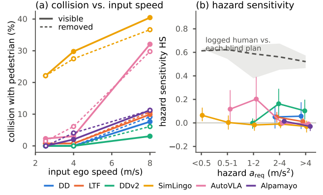
Fig. 3. Collision and hazard sensitivity. (a) Contact between the plan and the pedestrian’s logged future, at the logged speed and at counterfactual input speeds; solid: pedestrian visible, dashed: removed. (b) HS against the hazard level a_{\text{req}} (mean, 95% CI, bins with \geq 8 units; points dodged within a bin, and a policy appears only where it has enough units). Dashed: the logged human trajectory scored against each policy’s own blind plan, averaged over policies; band: the range across the six.
