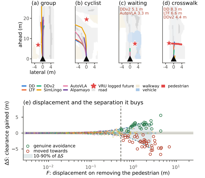
Fig. 5. Four right-hand-drive cases, and displacement against the separation it buys. (a–d) Ego at the origin, the VRU’s logged future dashed from the star, and DiffusionDriveV2’s own BEV semantic head as the background; every policy receives the frame’s logged navigation, so the turns are commanded. (a) Clearances 0.3–0.9 m. (b) SimLingo passes at 3.2 m, the other five at 6.7–10 m. (c, d) The departing policies and their planned distances are named in the panel; Boston departure rates are DiffusionDriveV2 81%, AutoVLA 9%, DiffusionDrive 2.8%. (e) Every policy–scene cell of the 246 Singapore scenes: F against \Delta S ; band: the 10–90% spread of \Delta S per F bin; dashed line: F = 0.5 m.
