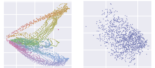
(a) Graph data representations. Analogous colors are time-of-day-adjacent. (b) Time-series data representations. Each point refers to a sensor in \mathcal{V} . Fig. 7. Visualization of CLEAR representations by principal component analysis.
