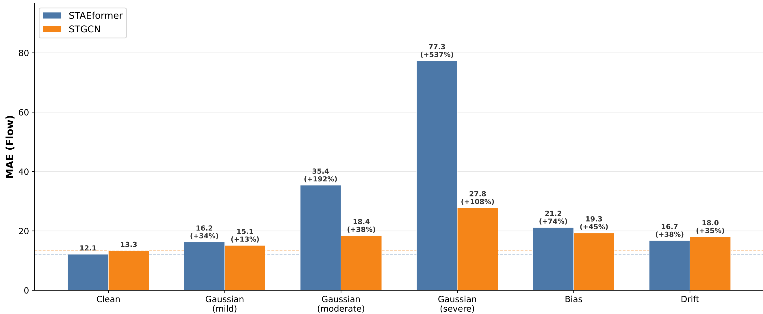
Baseline Prediction Degradation Under Sensor Noise (30% of sensors corrupted)
