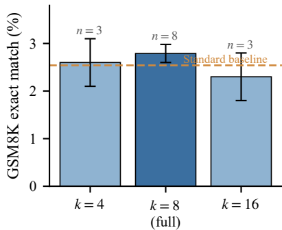
(a) Slot-count sweep
