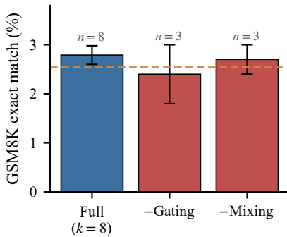
(b) Component ablation
