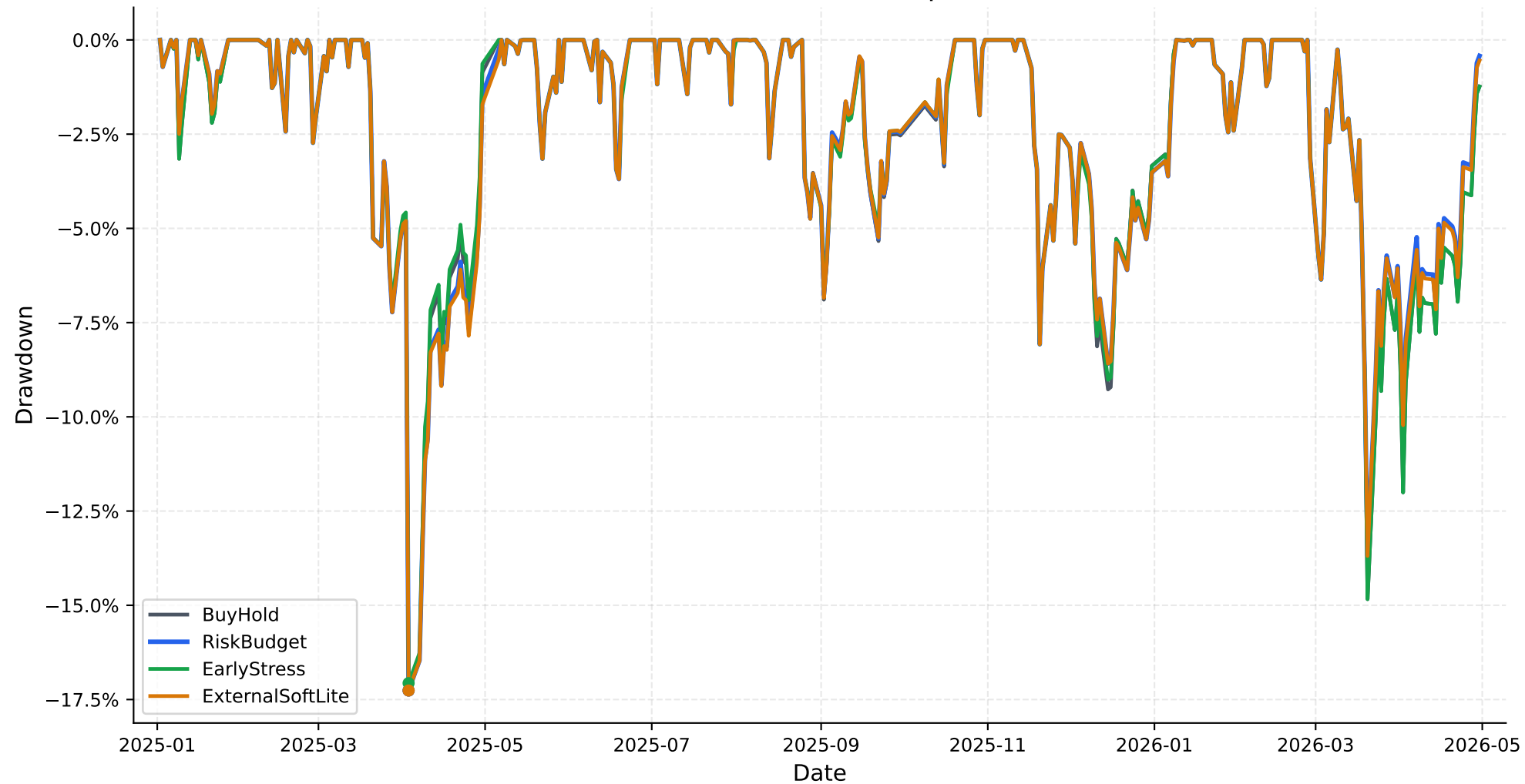
Drawdown Curve Comparison
