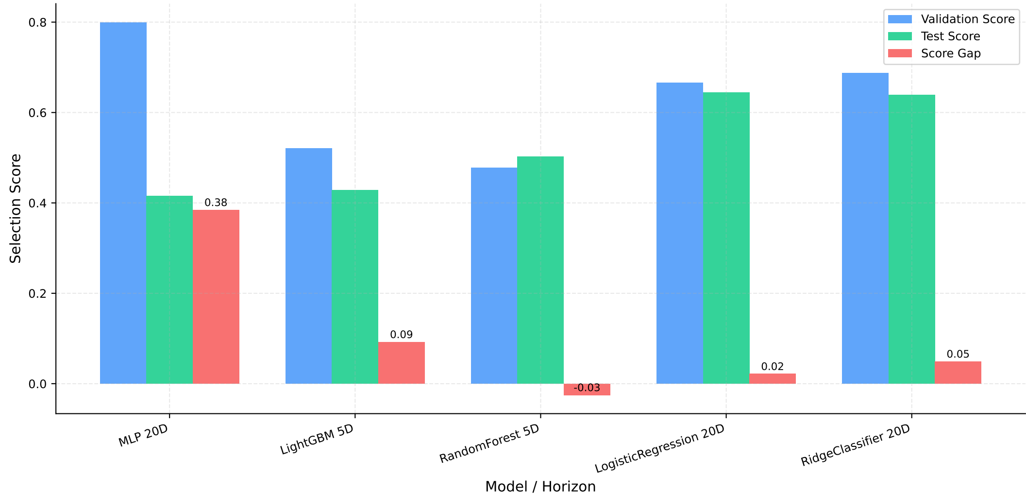
Validation-Test Stability Gap
