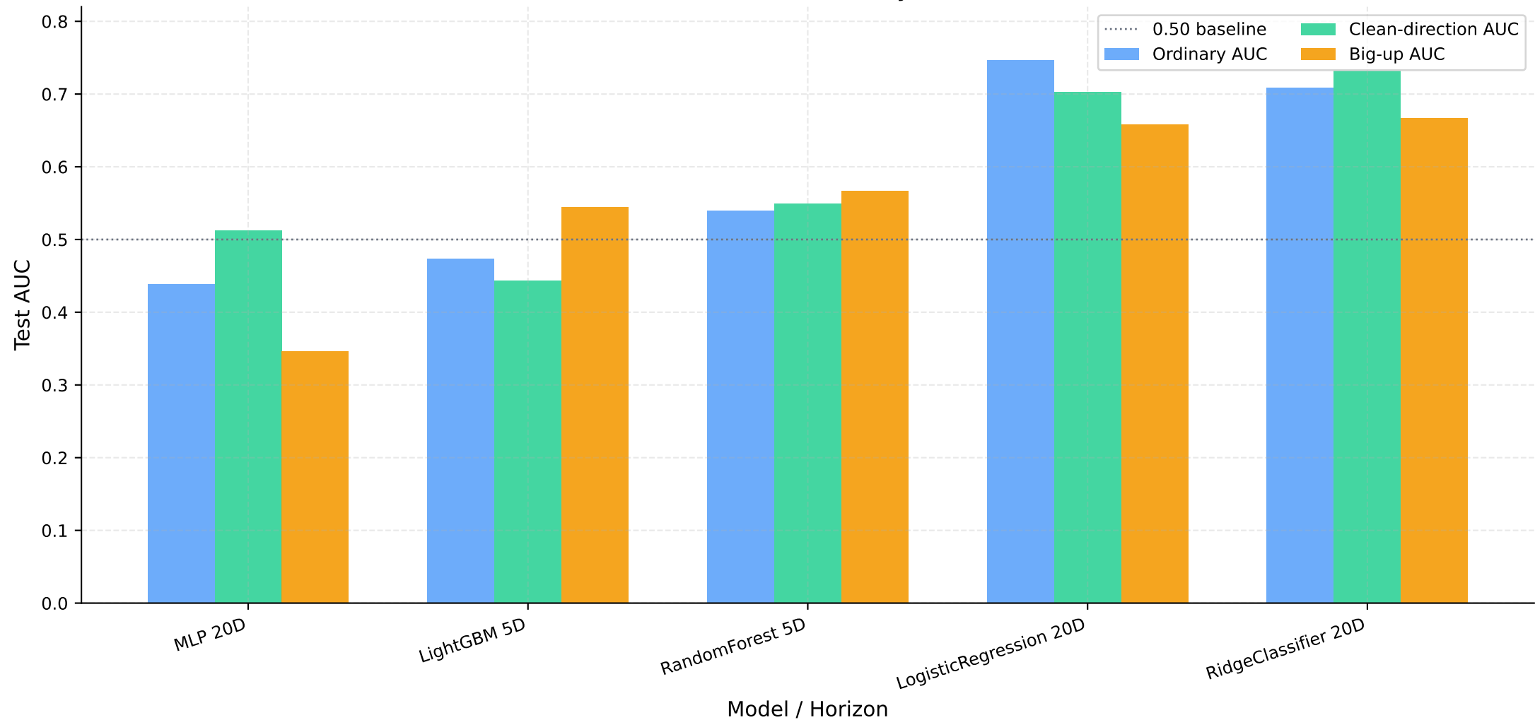
Test Prediction AUC by Model
