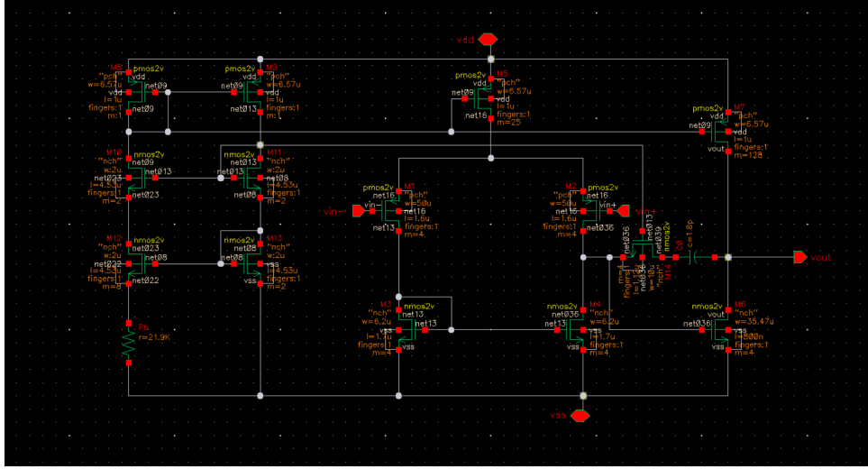
Figure 8: Complete OTA Schematic
