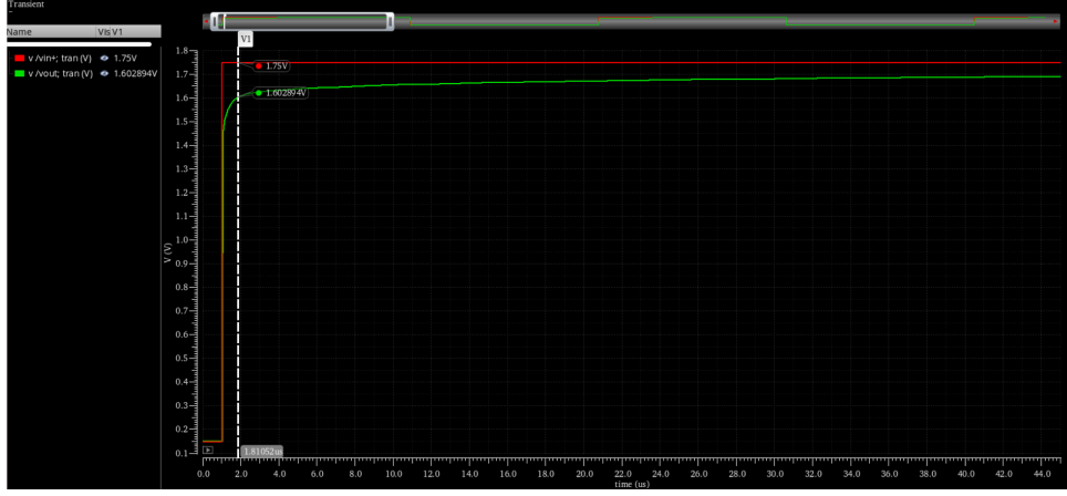
Figure 12: Output voltage's slow response when V_{cm} > 1.6V
