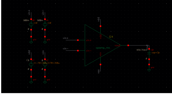
Figure 19: Open-Loop Configuration for V_{cm,q}
