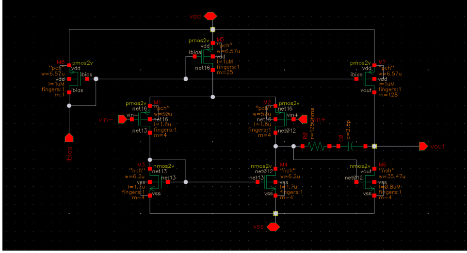
Figure 6: Optimized Core Schematic
