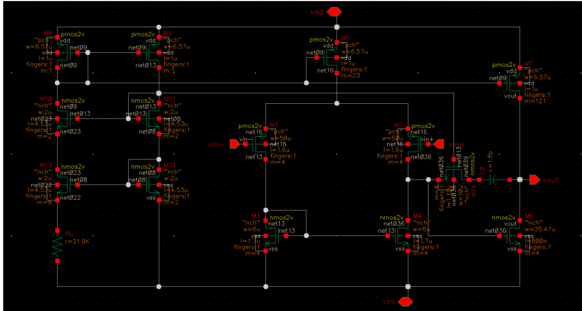
Figure 24: Final Optimized OTA Schematic
