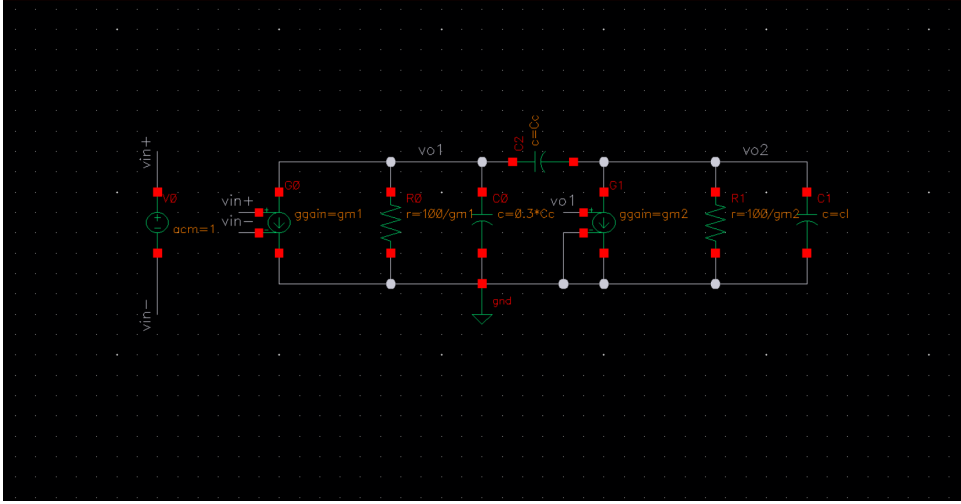
Figure 2: Small-Signal Model for the AC Simulation
