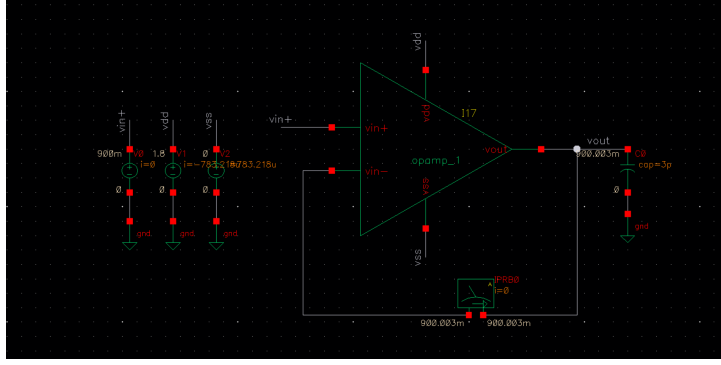
Figure 11: Slew Rate & Transient Response Testbench
