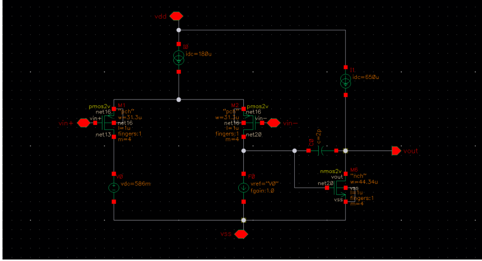
Figure 3: STB Simulation Setup for M2/M6 Verification
