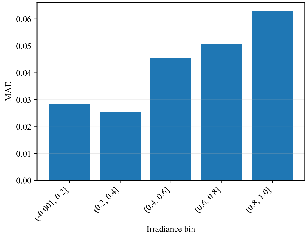
(b) Error by irradiance
