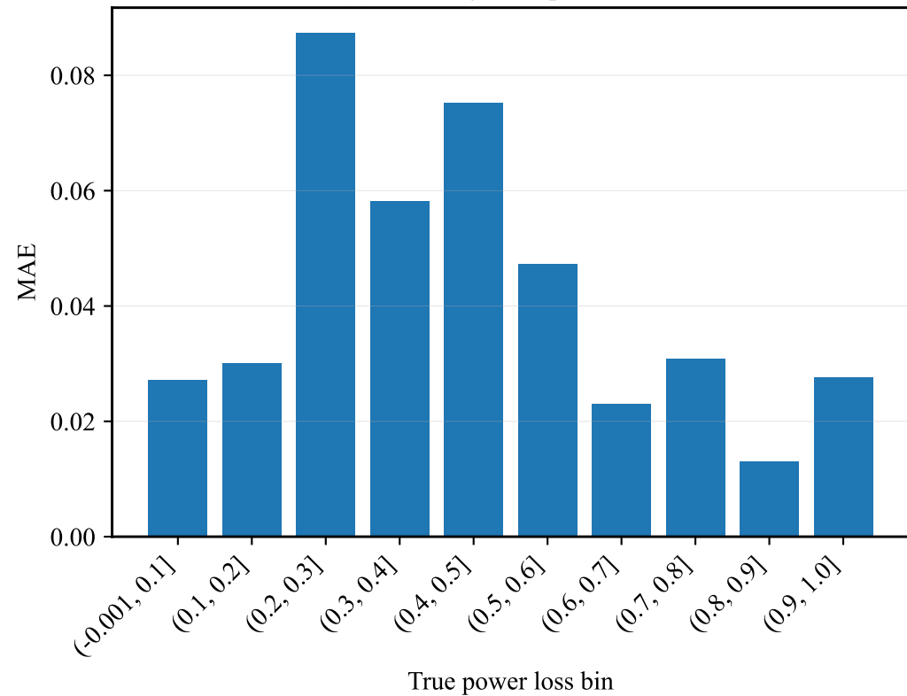
(a) Error by true power loss
