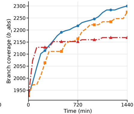
Forked-daapd
