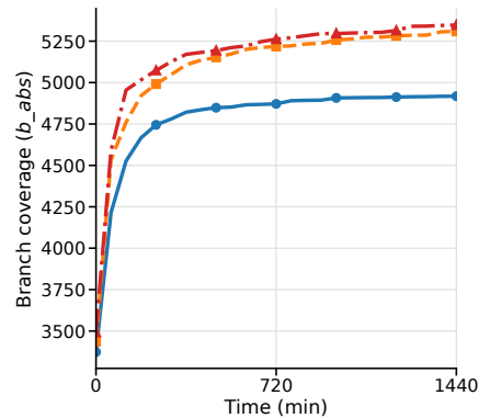
Kamailio
