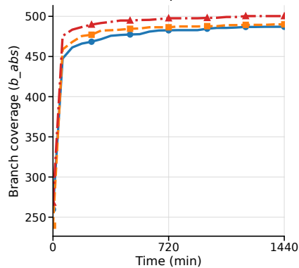
Live555
