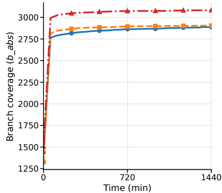
Live555
