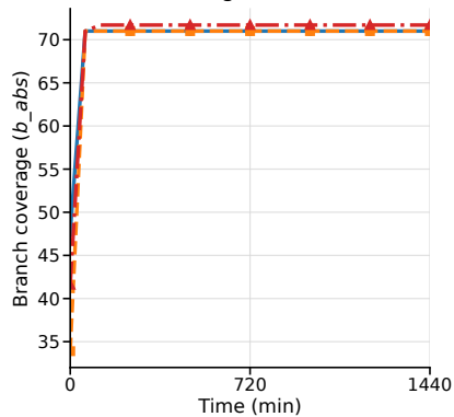
Exim
