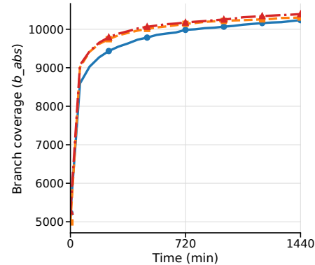
Kamailio
