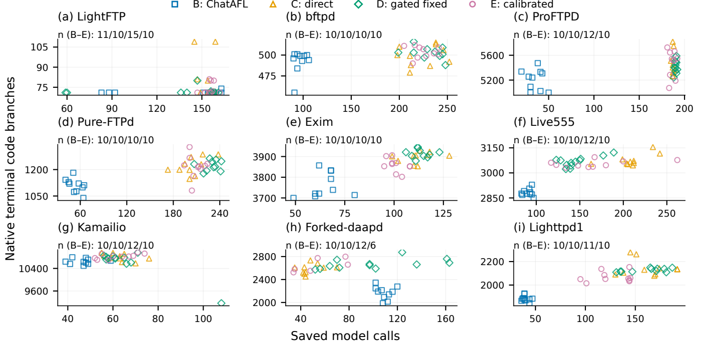
Figure 9: Saved model-call counters versus native terminal branch coverage for the same 371 B–E observations as Fig. 8. Each marker represents a run; no regression, Pareto frontier, or missing usage is inferred. Separate target scales preserve the different program coverage surfaces. Call counts do not measure token expenditure or CPU-hours.
