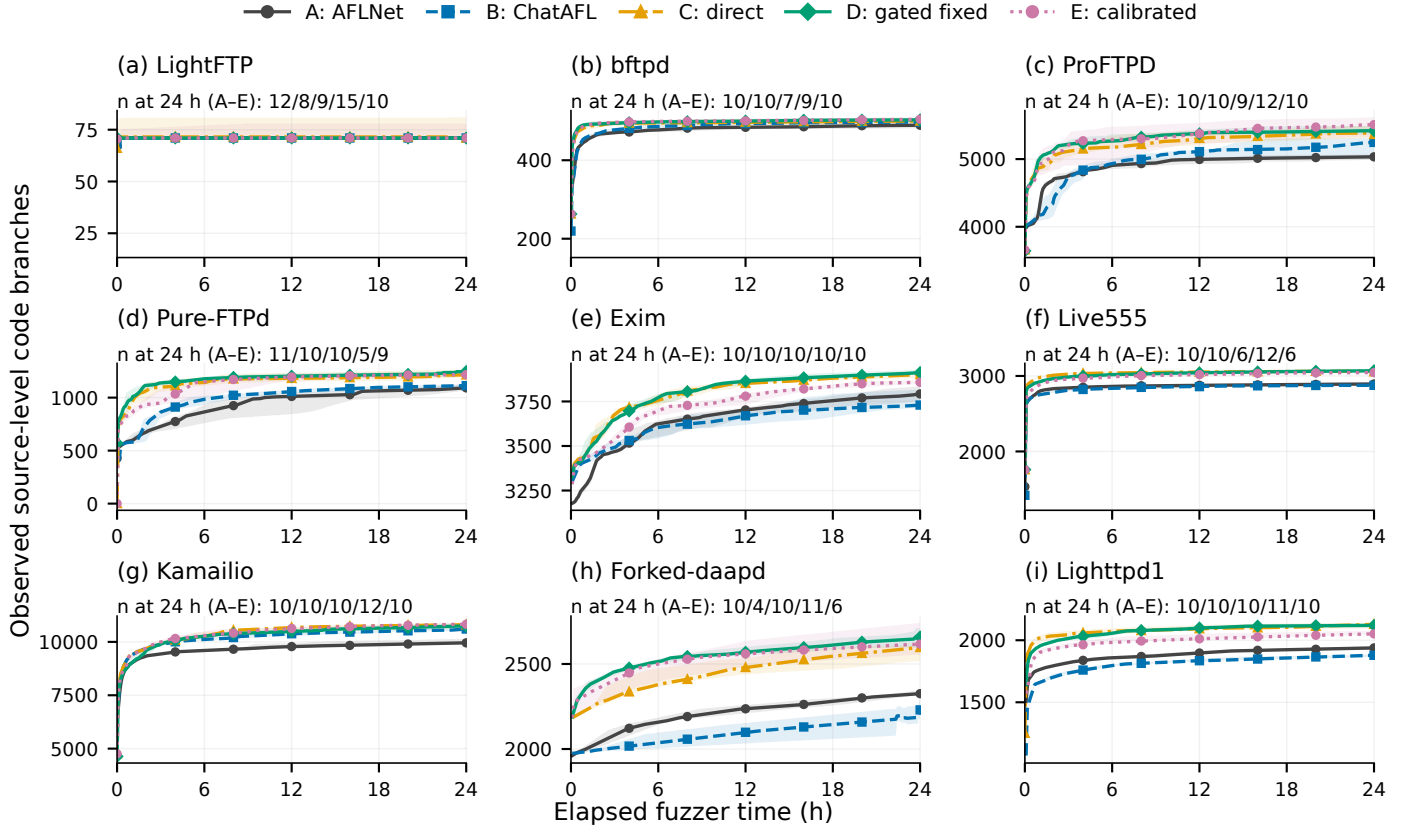
Figure 5: Observed A–E code-branch trajectories from 465 archives. Time is measured from each fuzzer_stats start time. Lines are medians and shaded regions are interquartile ranges, computed on a five-minute grid by linear interpolation only between recorded observations. A run contributes neither before its first observation nor after its last; the actual contributing n at 24 hours is shown in A–E order. The plot displays 0–24 hours without imposing a completed 24-hour campaign on interrupted runs. Full time-dependent denominators accompany the figure data; the nominal target remains N = 10 . All 45 main target–arm combinations are represented, including ten E–bftpd archives. Native pipeline/build comparability remains unverified; these curves are descriptive, and shaded ranges are not confidence intervals.
