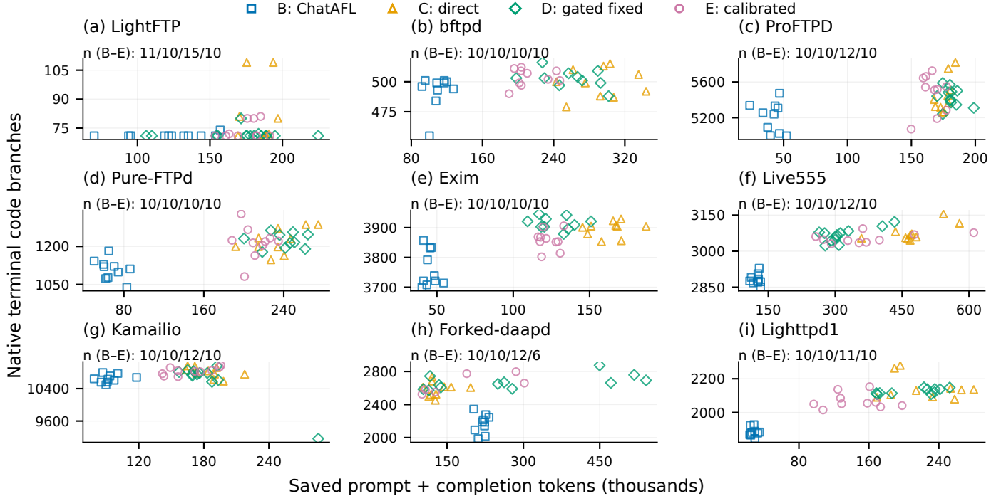
Figure 8: Saved token counters versus native terminal code coverage, with one marker per B–E archive (371 observations). Token usage is the saved prompt-plus-completion count, expressed in thousands; individual observations show the available dispersion without imposing a fitted efficiency frontier. Different targets have separate axes; all 36 B–E target–arm combinations have saved counters, including ten E–bftpd archives. AFLNet lacks a comparable saved counter and is not assigned a synthetic zero. Horizons and build provenance are not matched, and final counters may lag the event stream. This is a descriptive cost–coverage view, not reconciled billing or a cost-matched causal comparison.
