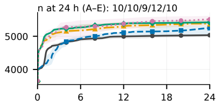
(f) Live555
