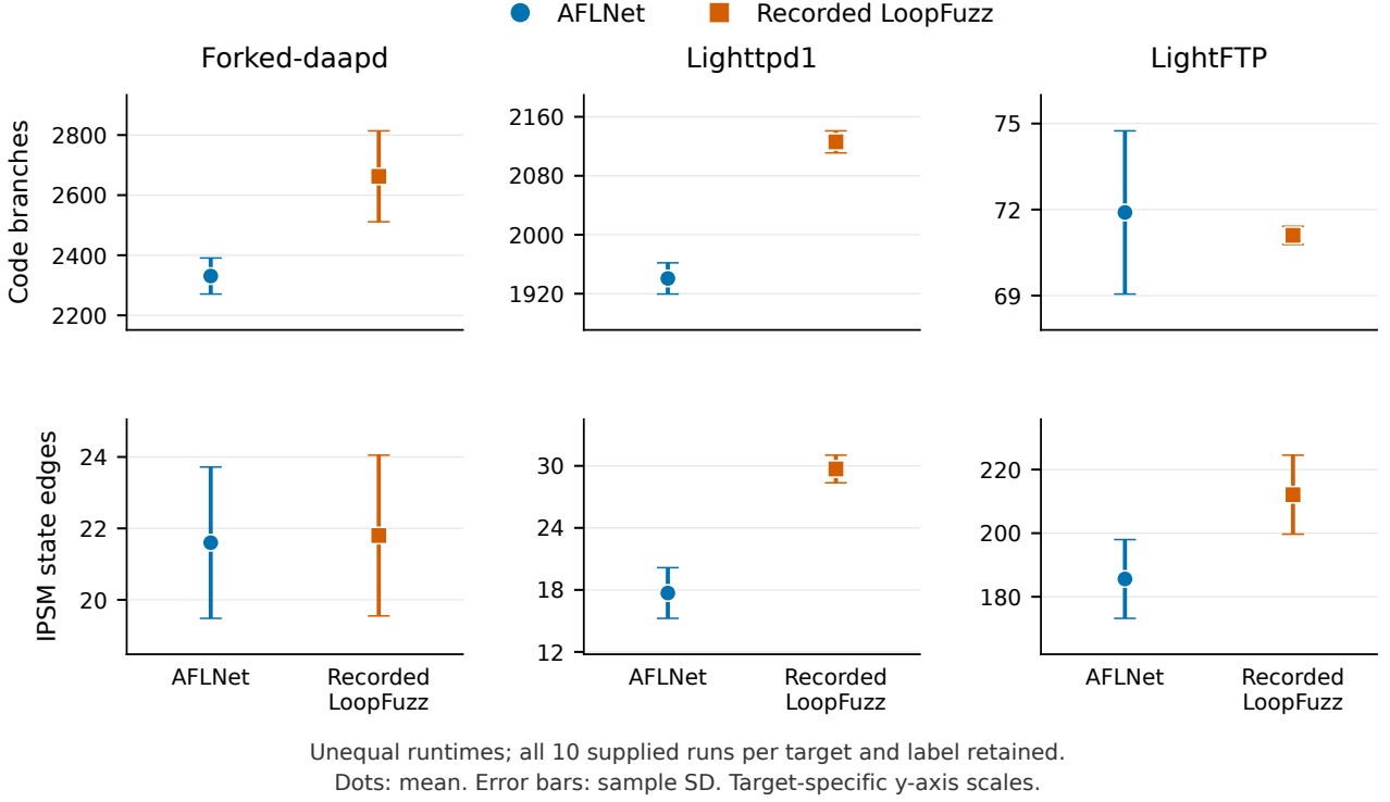
Figure 1: Observed native terminal code-branch and IPSM state-edge counts for the three motivating targets (mean and sample standard deviation; ten supplied runs per target and label). All runs, including interruptions, are retained. Runtime and provenance differences prevent a matched-horizon causal interpretation. This figure tests the earlier narrative against current observations: it does not assert that all three hypothesized mismatch types were reproduced.
