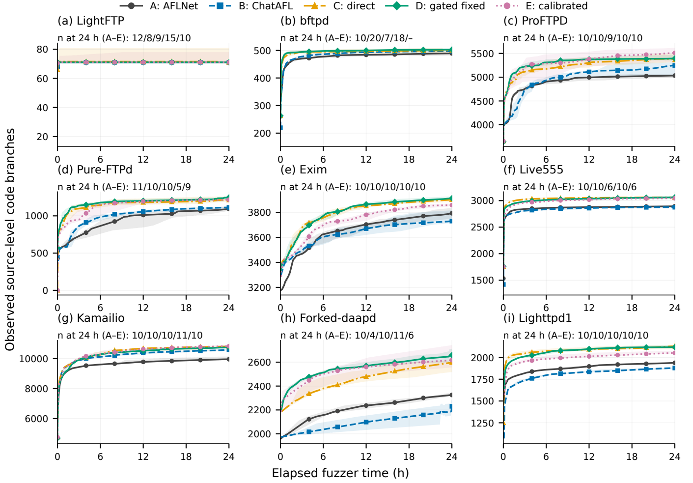
Figure 5: Observed A-E code-branch trajectories from 469 archives. Time is measured from each fuzzer_stats start time. Lines are medians and shaded regions are interquartile ranges, computed on a five-minute grid by linear interpolation only between recorded observations. A run contributes neither before its first observation nor after its last; the actual contributing n at 24 hours is shown in A-E order. The plot displays 0–24 hours without imposing a completed 24-hour campaign on interrupted runs. Full time-dependent denominators accompany the figure data; the nominal target remains N = 10 . Missing E-bftpd is omitted. Native pipeline/build comparability remains unverified; these curves are descriptive, and shaded ranges are not confidence intervals.
