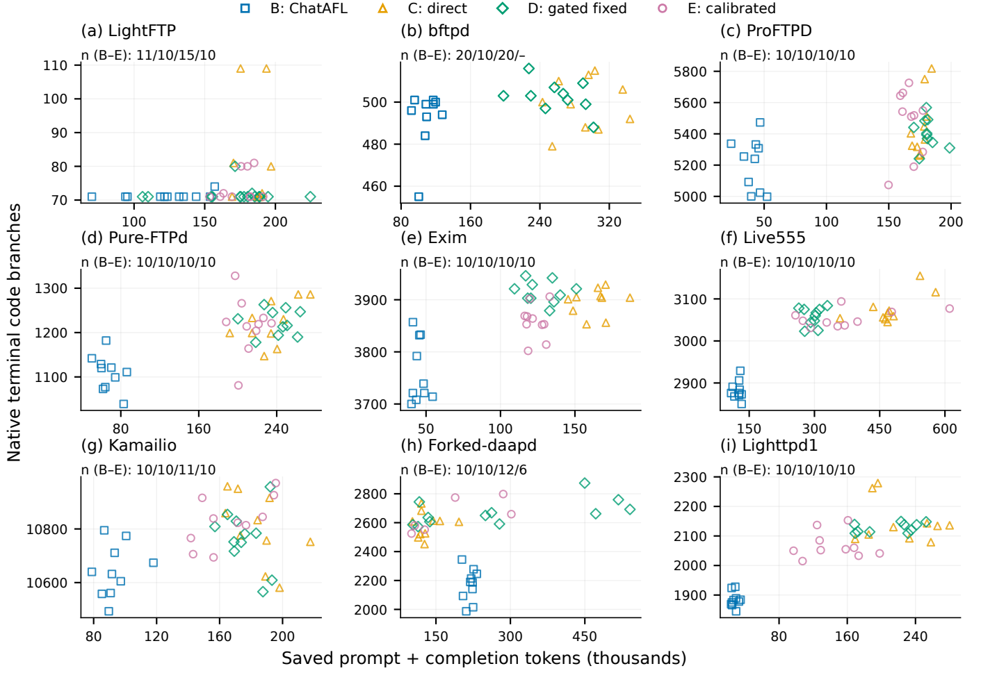
Figure 8: Saved token counters versus native terminal code coverage, with one marker per B–E archive (375 observations). Token usage is the saved prompt-plus-completion count, expressed in thousands; individual observations show the available dispersion without imposing a fitted efficiency frontier. Different targets have separate axes, and missing E–bftpd is omitted. AFLNet lacks a comparable saved counter and is not assigned a synthetic zero. Horizons and build provenance are not matched, and final counters may lag the event stream. This is a descriptive cost–coverage view, not reconciled billing or a cost-matched causal comparison.
