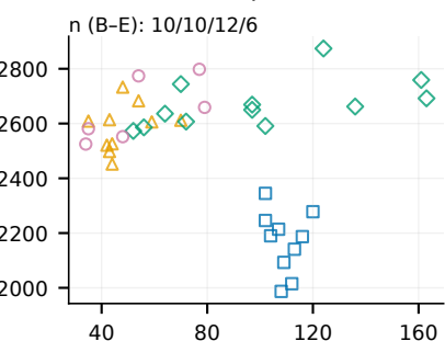
(h) Forked-daapd
