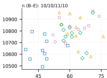
(g) Kamailio
