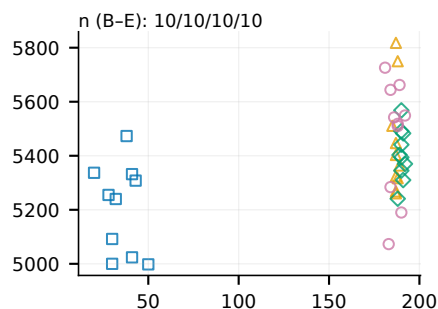
(f) Live555
