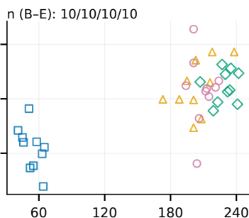
(g) Kamailio
