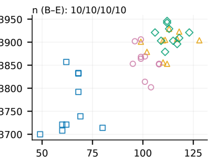
(h) Forked-daapd
