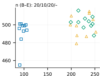
(e) Exim
